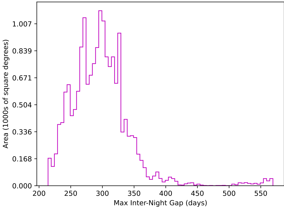
ddf_acor_sf15_lsf20_lsr20_v3.4_10yrs WFD z band: Max Inter-Night Gap
