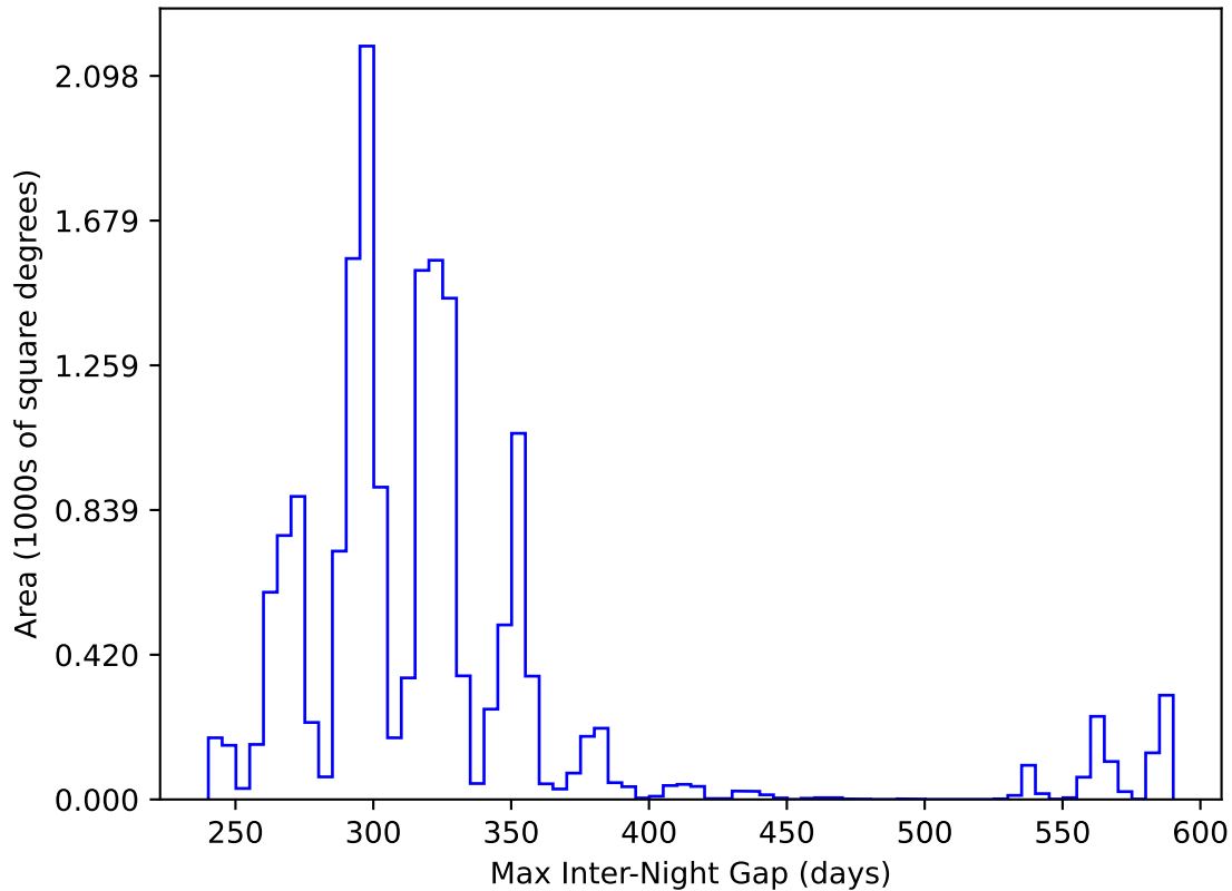
ddf_acor_sf15_lsf20_lsr20_v3.4_10yrs WFD y band: Max Inter-Night Gap
