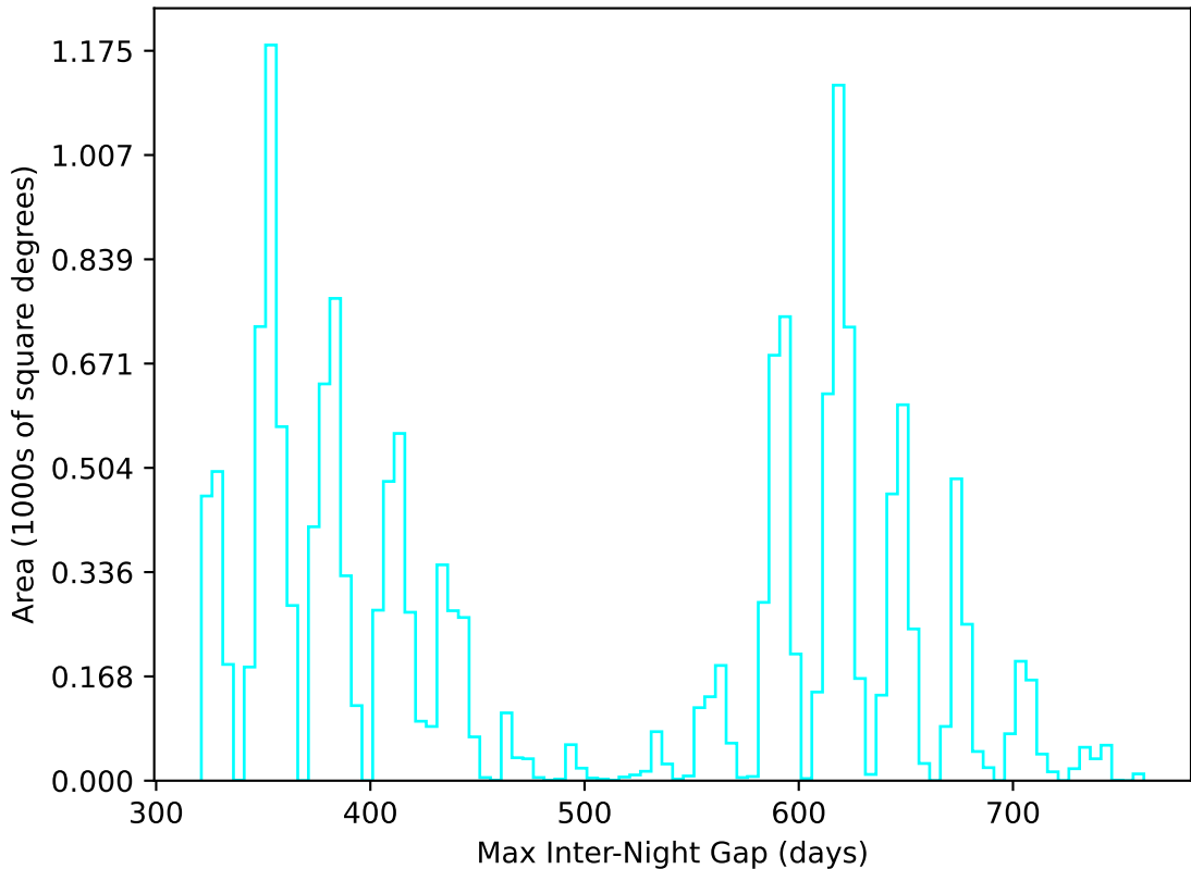
ddf_acor_sf15_lsf20_lsr20_v3.4_10yrs WFD u band: Max Inter-Night Gap
