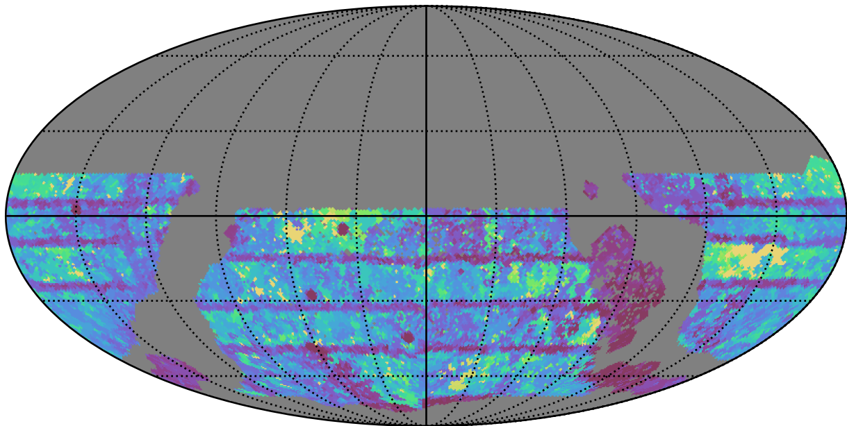
ddf_acor_sf15_lsf20_lsr20_v3.4_10yrs WFD r band: Max Inter-Night Gap
