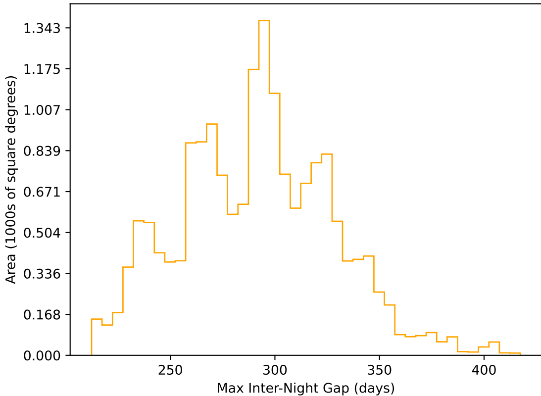
ddf_acor_sf15_lsf20_lsr20_v3.4_10yrs WFD r band: Max Inter-Night Gap
