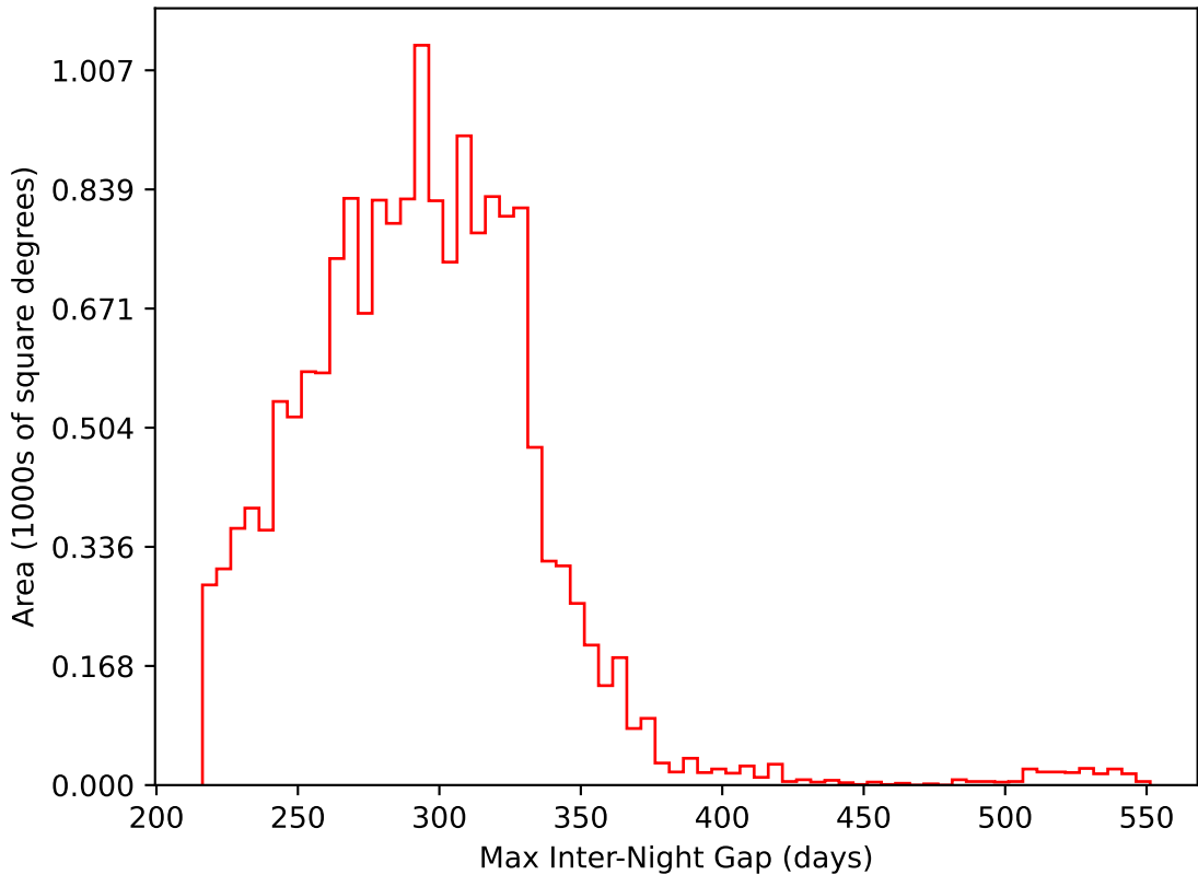
ddf_acor_sf15_lsf20_lsr20_v3.4_10yrs WFD i band: Max Inter-Night Gap
