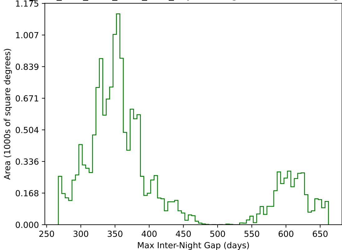
ddf_acor_sf15_lsf20_lsr20_v3.4_10yrs WFD g band: Max Inter-Night Gap
