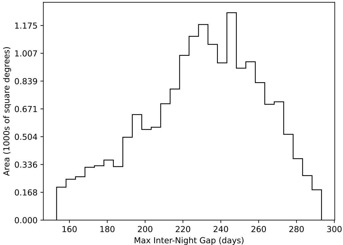
ddf_acor_sf15_lsf20_lsr20_v3.4_10yrs WFD all bands: Max Inter-Night Gap
