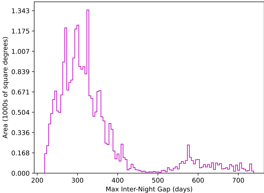
ddf_acor_sf15_lsf20_lsr20_v3.4_10yrs All sky z band: Max Inter-Night Gap
