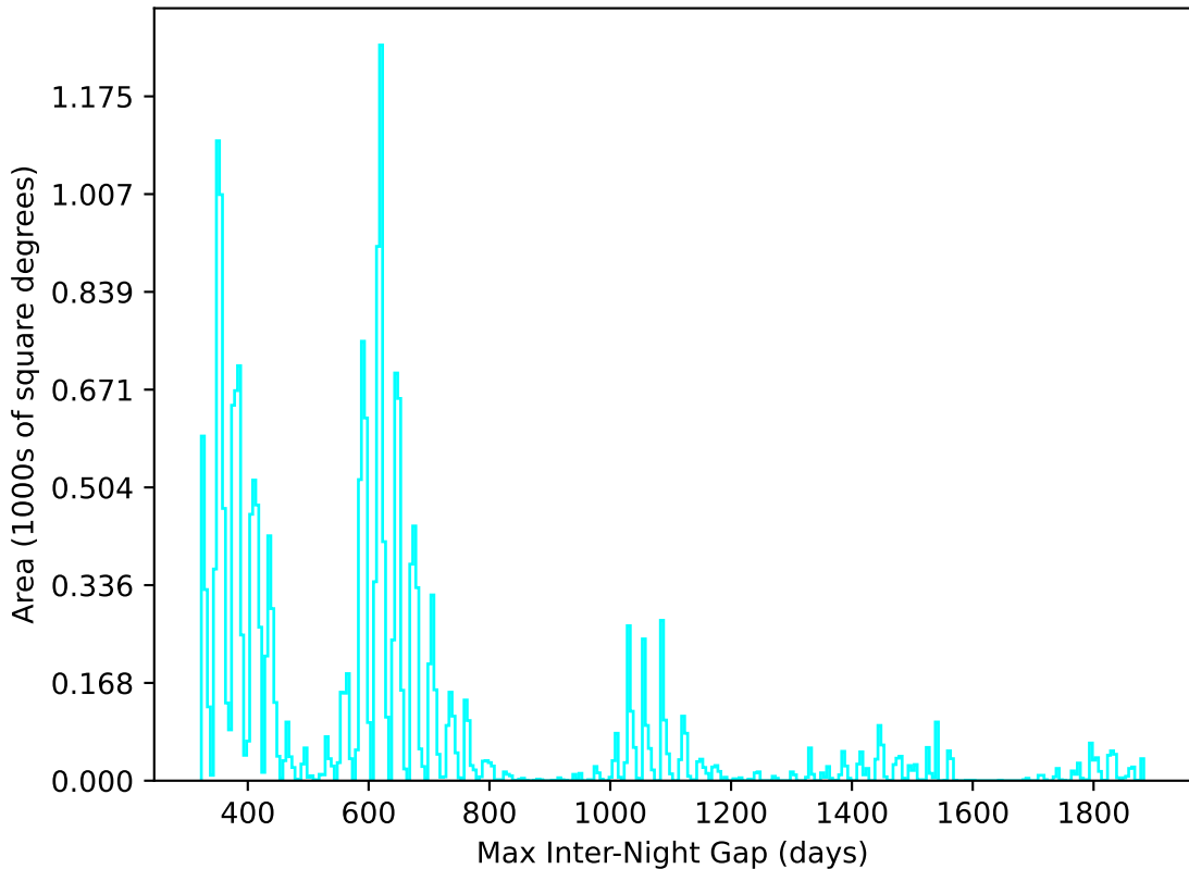
ddf_acor_sf15_lsf20_lsr20_v3.4_10yrs All sky u band: Max Inter-Night Gap
