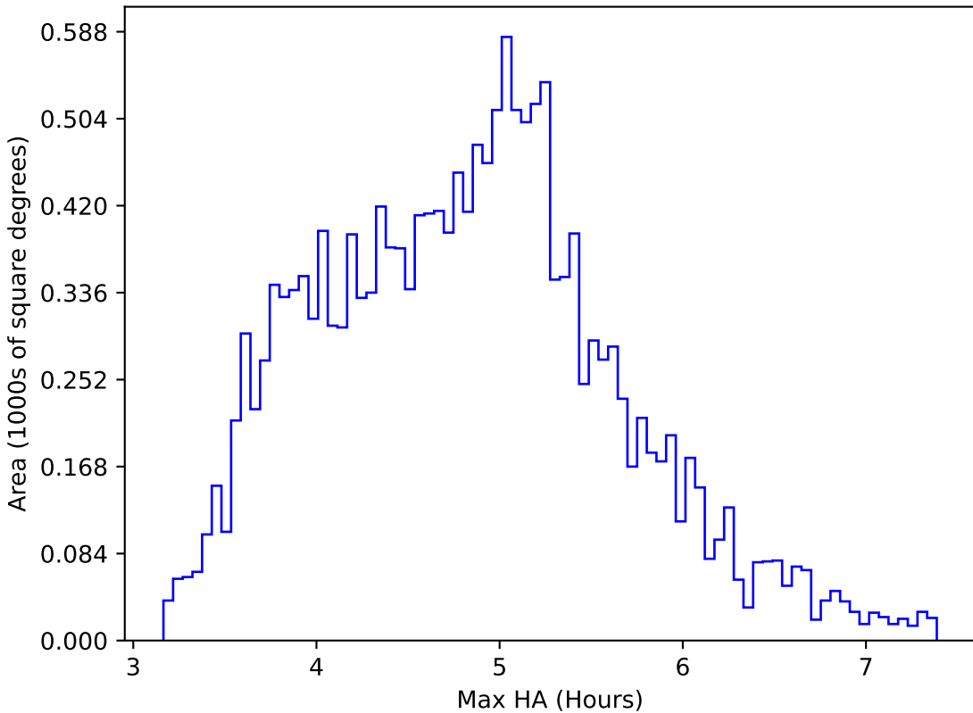
ddf_acor_sf15_lsf20_lsr20_v3.4_10yrs WFD z band: Max HA
