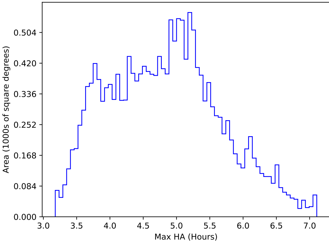
ddf_acor_sf15_lsf20_lsr20_v3.4_10yrs WFD i band: Max HA
