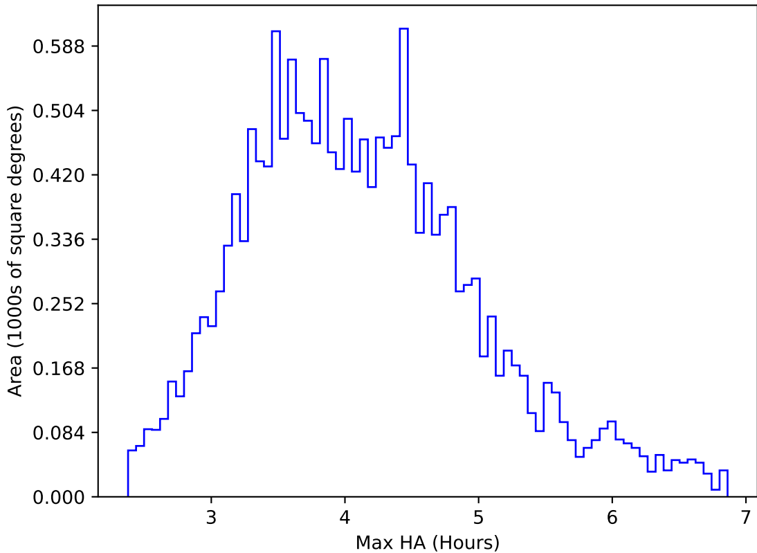
ddf_acor_sf15_lsf20_lsr20_v3.4_10yrs WFD g band: Max HA
