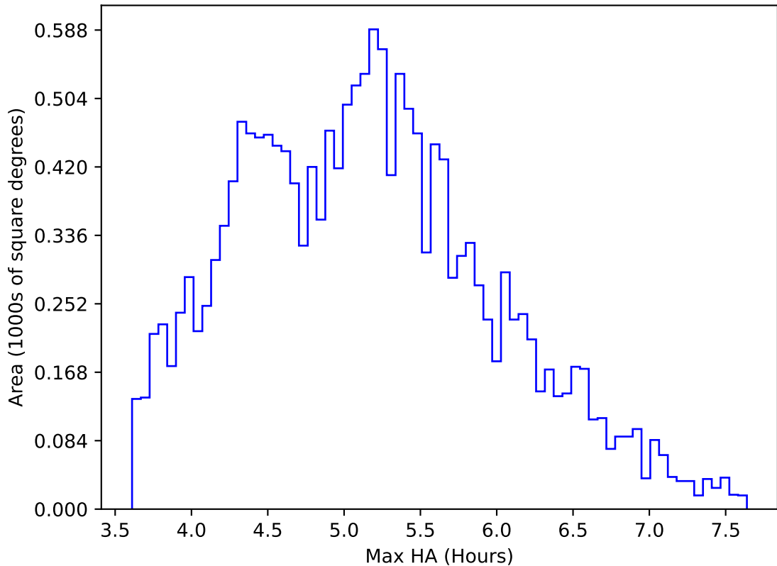
ddf_acor_sf15_lsf20_lsr20_v3.4_10yrs WFD all bands: Max HA
