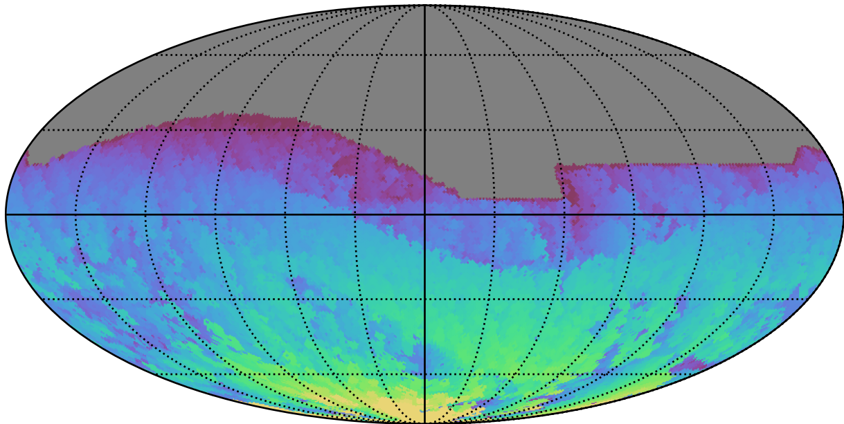
ddf_acor_sf15_lsf20_lsr20_v3.4_10yrs All sky z band: Max HA
