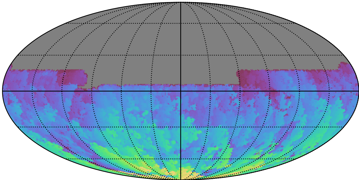
ddf_acor_sf15_lsf20_lsr20_v3.4_10yrs All sky u band: Max HA
