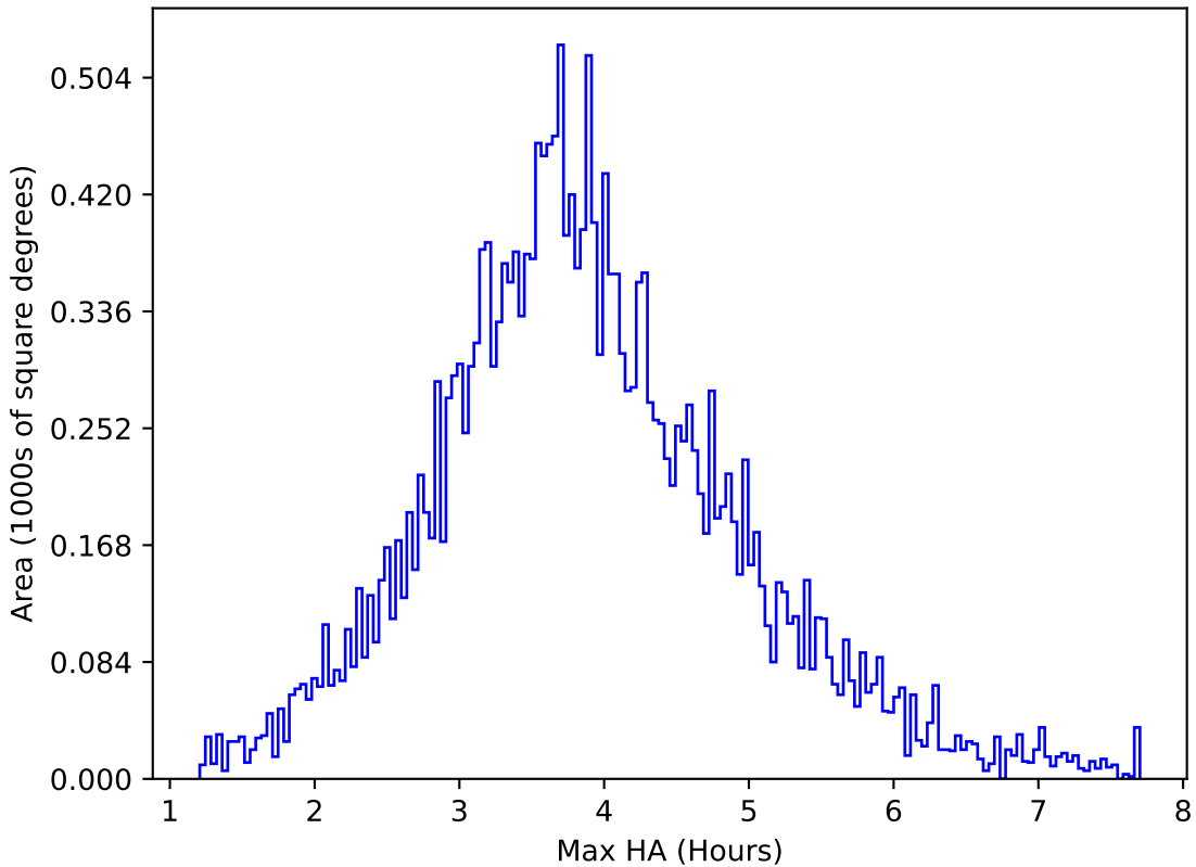
ddf_acor_sf15_lsf20_lsr20_v3.4_10yrs All sky u band: Max HA
