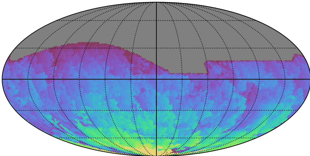
ddf_acor_sf15_lsf20_lsr20_v3.4_10yrs All sky r band: Max HA
