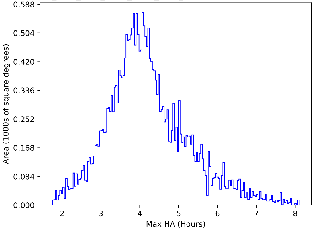
ddf_acor_sf15_lsf20_lsr20_v3.4_10yrs All sky r band: Max HA
