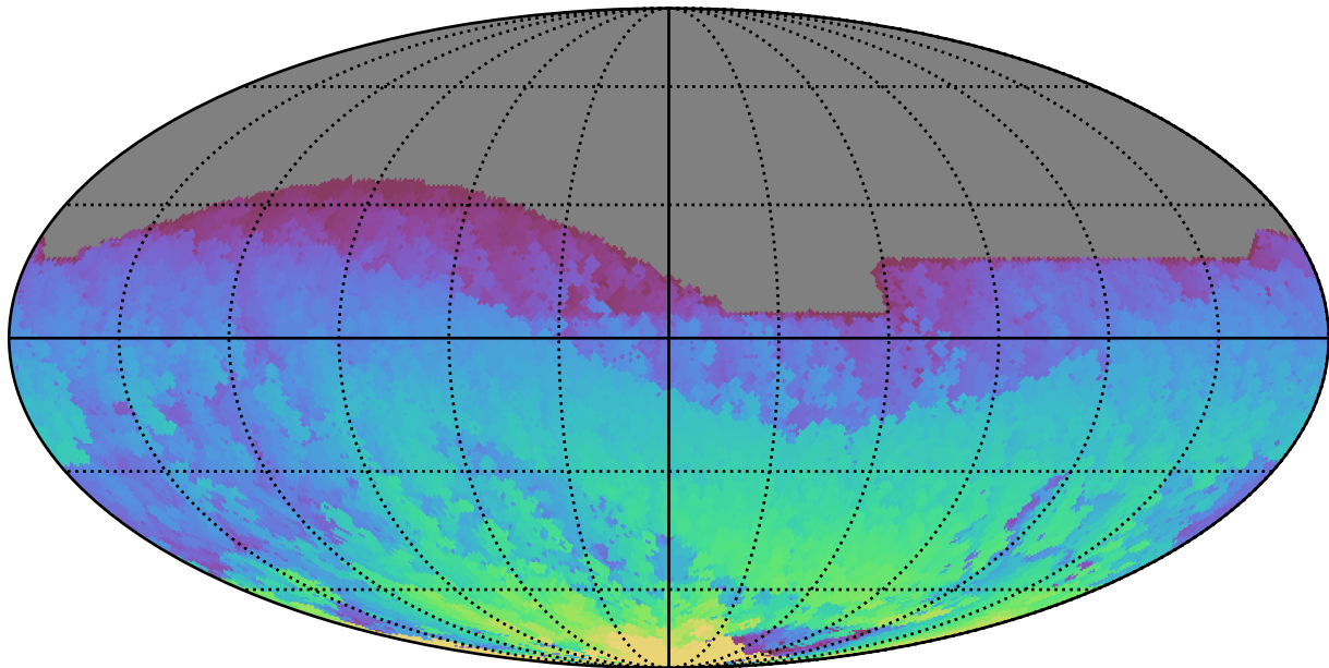
ddf_acor_sf15_lsf20_lsr20_v3.4_10yrs All sky i band: Max HA
