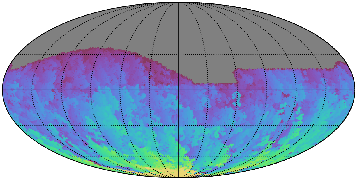
ddf_acor_sf15_lsf20_lsr20_v3.4_10yrs All sky g band: Max HA
