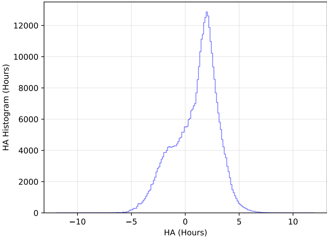
ddf_acor_sf15_lsf20_lsr20_v3.4_10yrs WFD y band: HA Histogram
