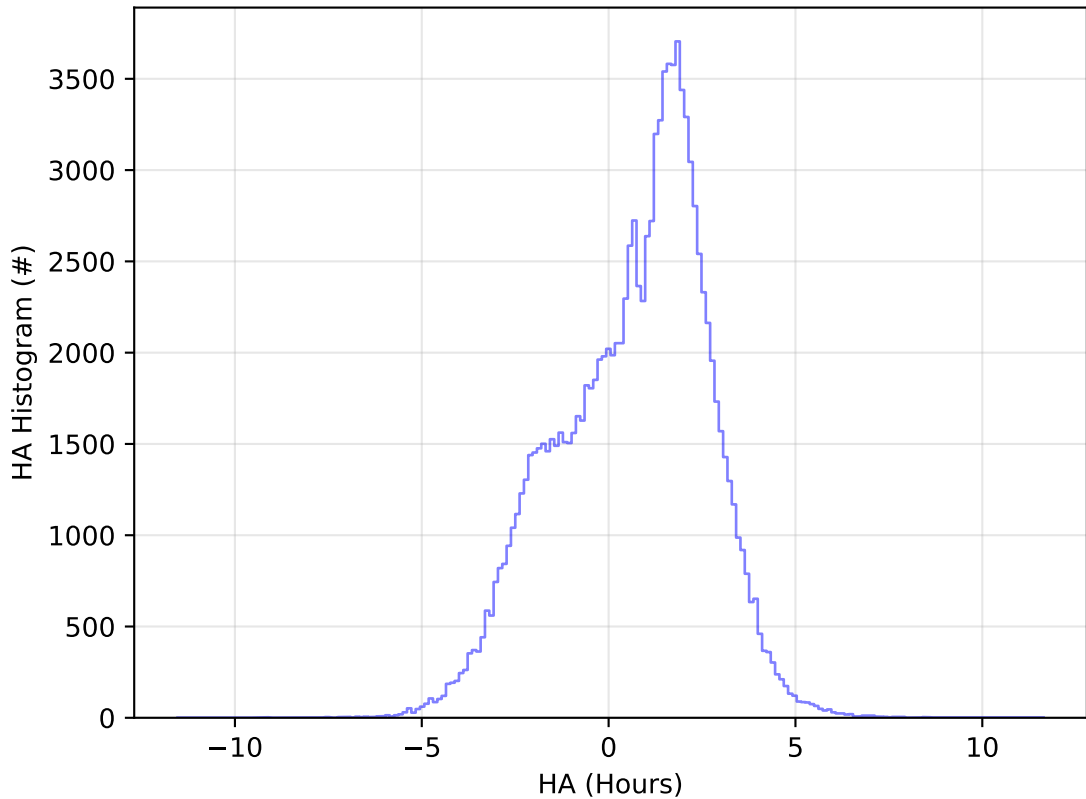
ddf_acor_sf15_lsf20_lsr20_v3.4_10yrs WFD u band: HA Histogram
