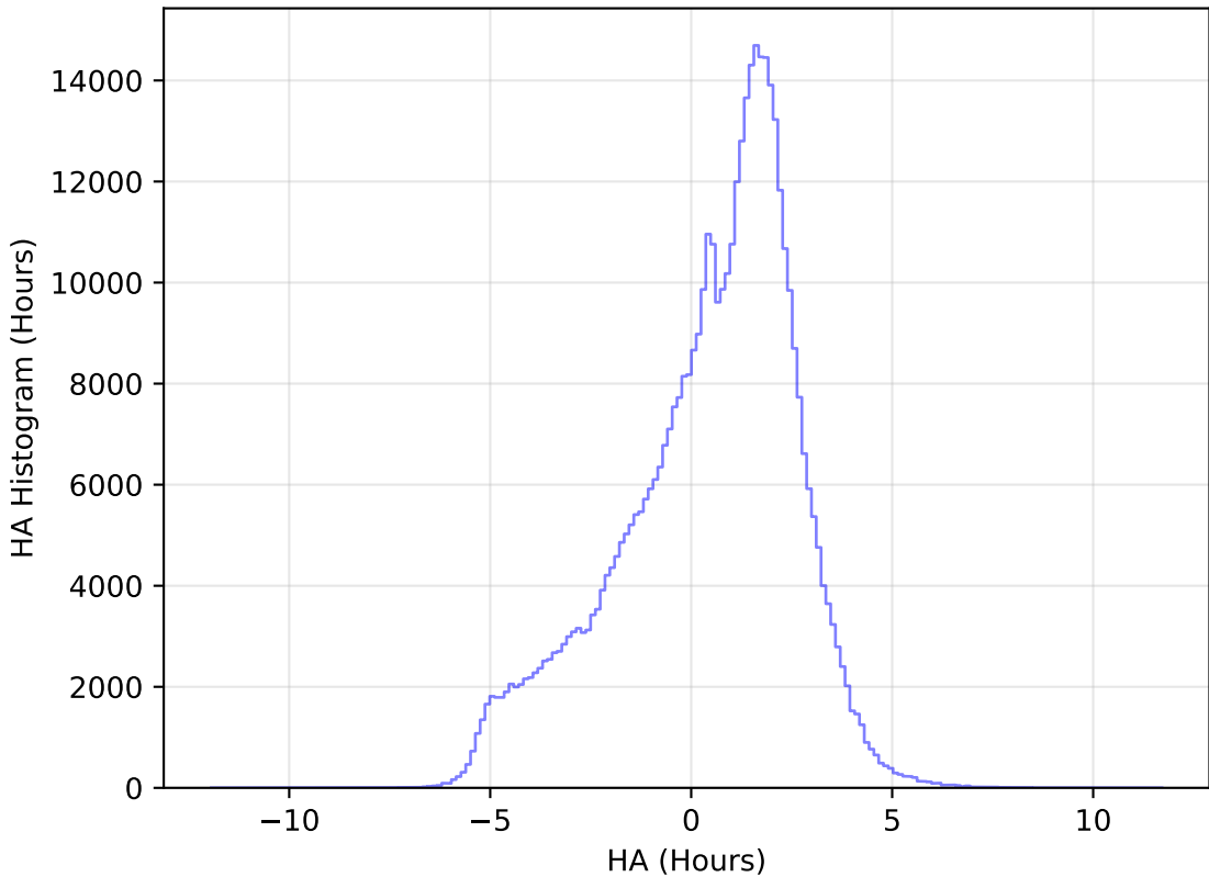
ddf_acor_sf15_lsf20_lsr20_v3.4_10yrs WFD r band: HA Histogram
