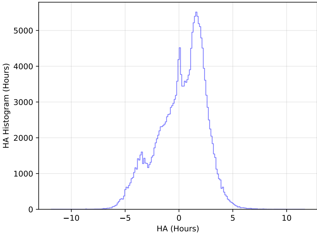
ddf_acor_sf15_lsf20_lsr20_v3.4_10yrs WFD g band: HA Histogram
