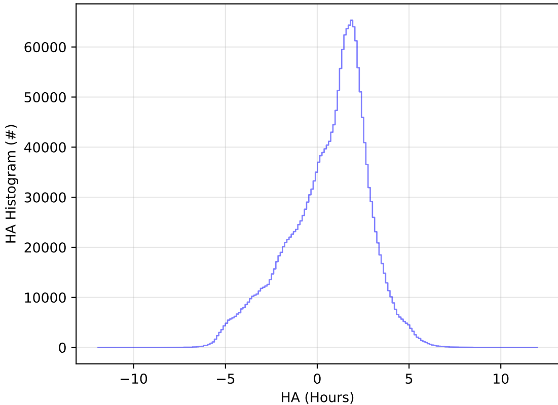
ddf_acor_sf15_lsf20_lsr20_v3.4_10yrs WFD all bands: HA Histogram
