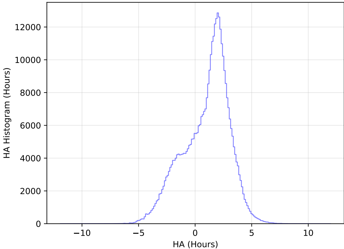
ddf_acor_sf15_lsf20_lsr20_v3.4_10yrs All sky y band: HA Histogram
