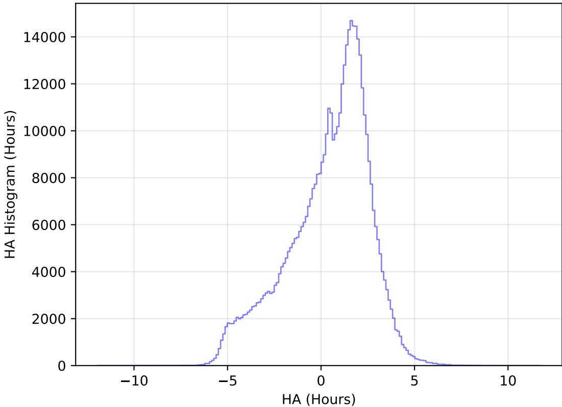
ddf_acor_sf15_lsf20_lsr20_v3.4_10yrs All sky r band: HA Histogram
