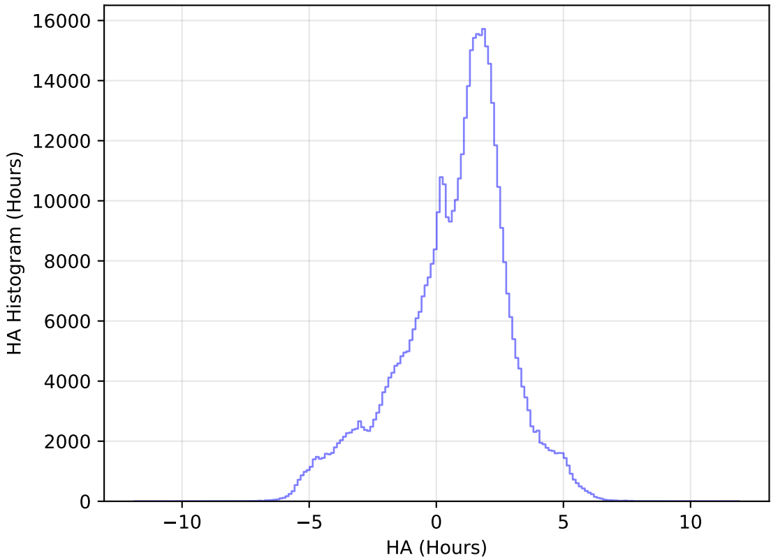
ddf_acor_sf15_lsf20_lsr20_v3.4_10yrs All sky i band: HA Histogram
