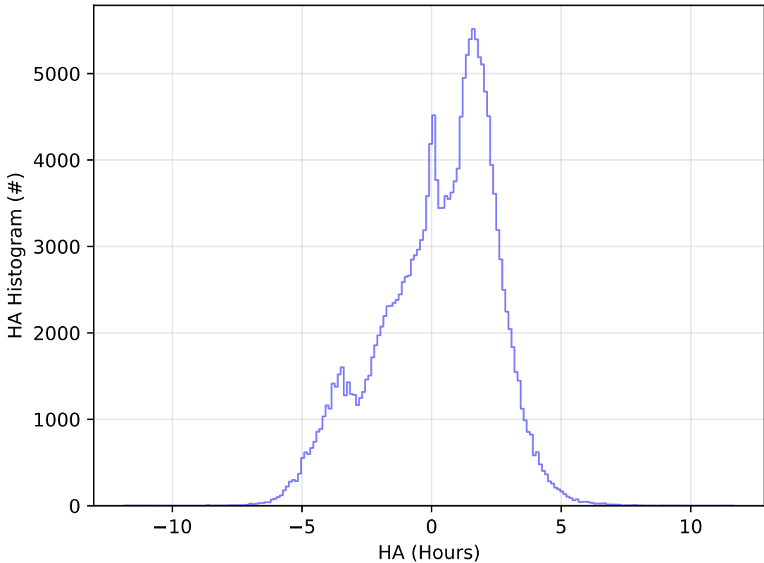
ddf_acor_sf15_lsf20_lsr20_v3.4_10yrs All sky g band: HA Histogram
