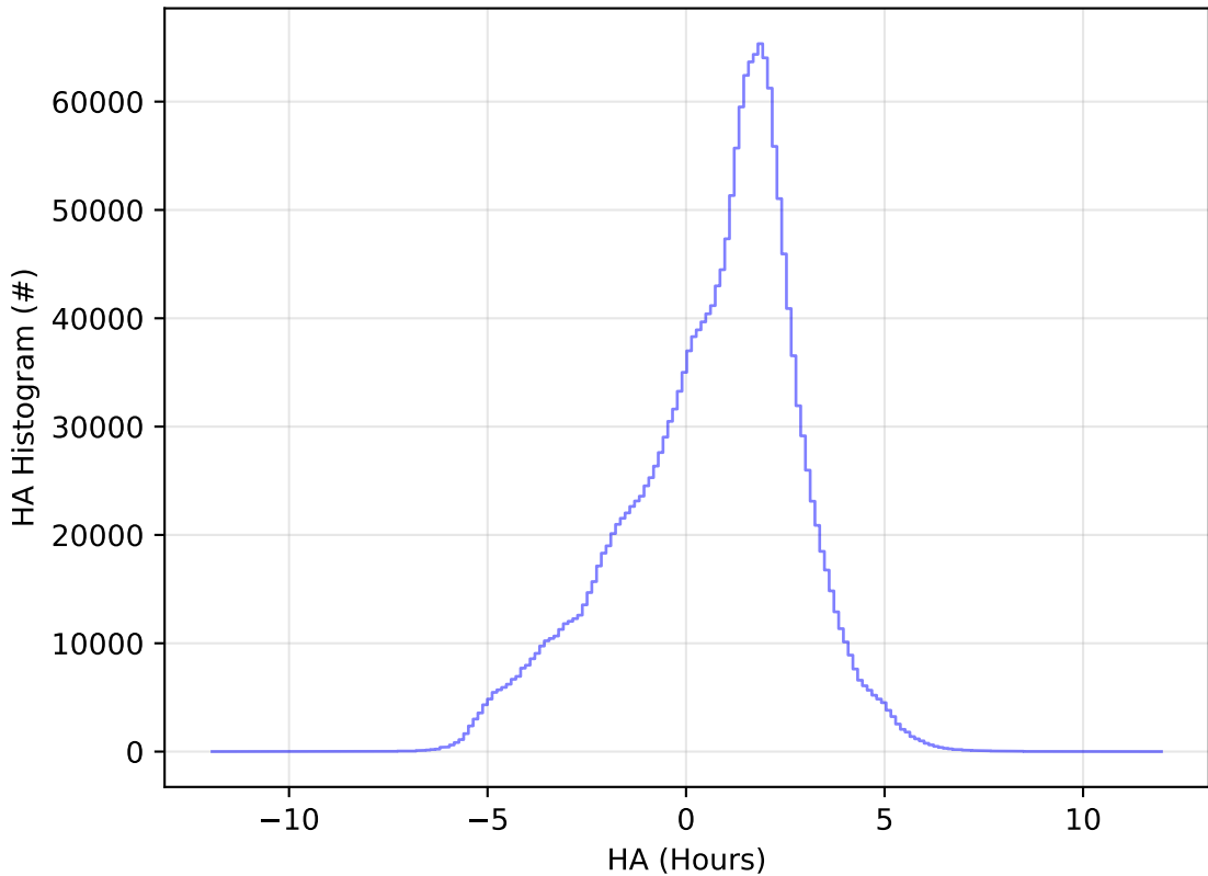
ddf_acor_sf15_lsf20_lsr20_v3.4_10yrs All sky all bands: HA Histogram
