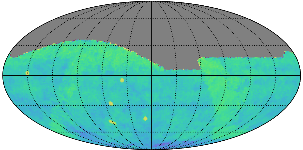
ddf_acor_sf15_lsf20_lsr20_v3.4_10yrs gri All sky: Fraction of visits in pairs (10-60 min)
