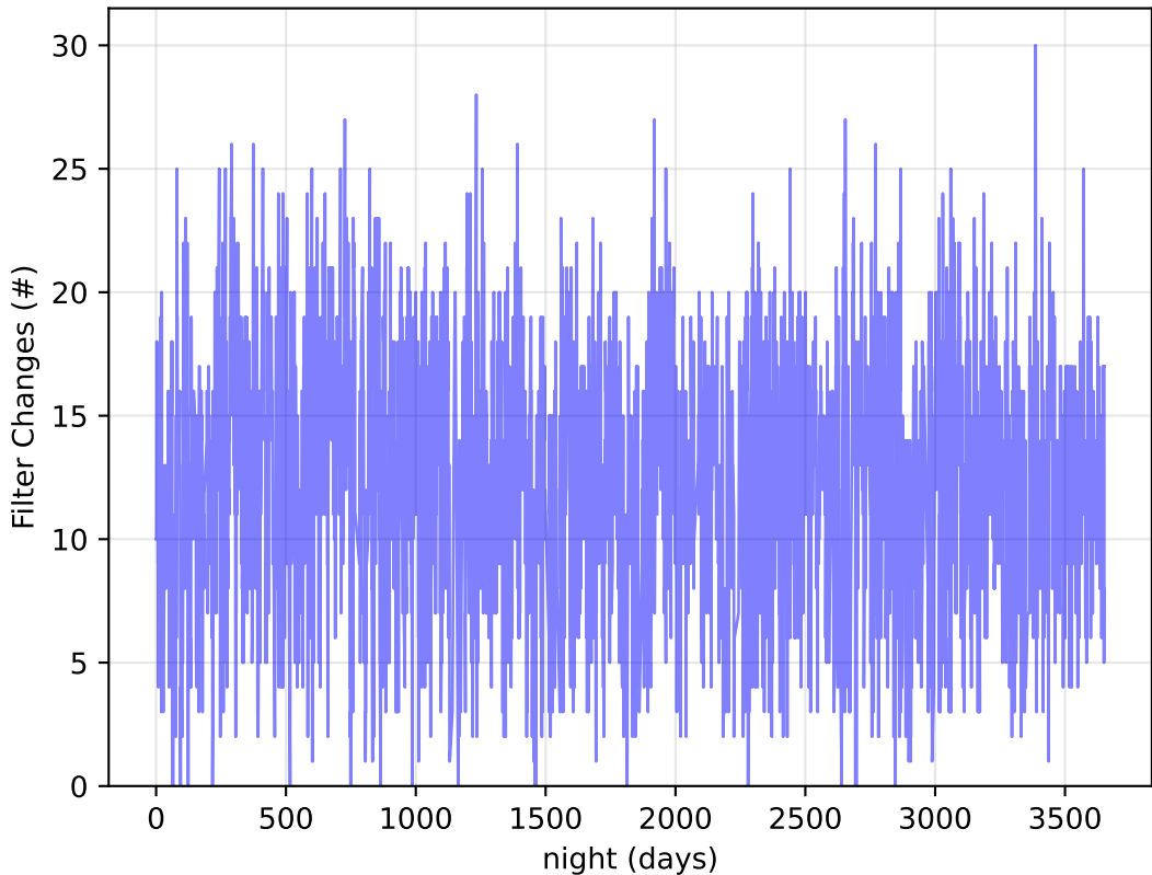
ddf_acor_sf15_lsf20_isr20_v3.4_10yrs Per Night: Filter Changes
