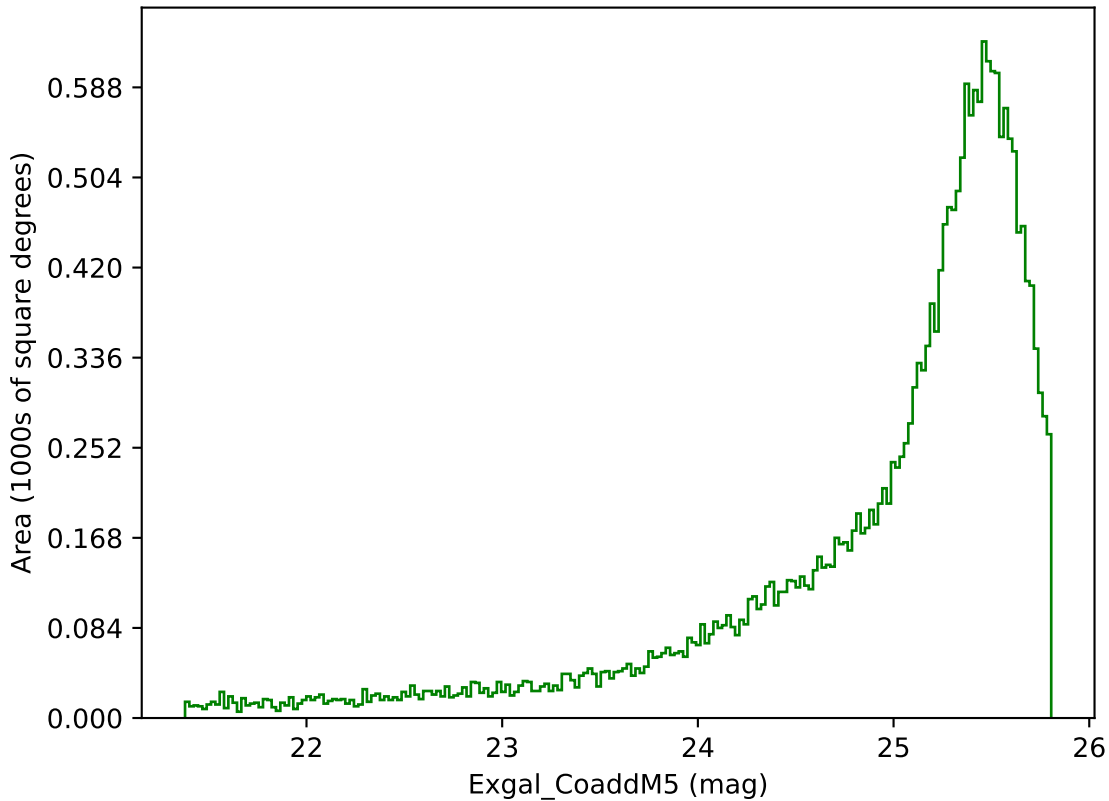
ddf_acor_sf15_lsf20_lsr20_v3.4_10yrs Yr 1 g band: Exgal_CoaddM5
