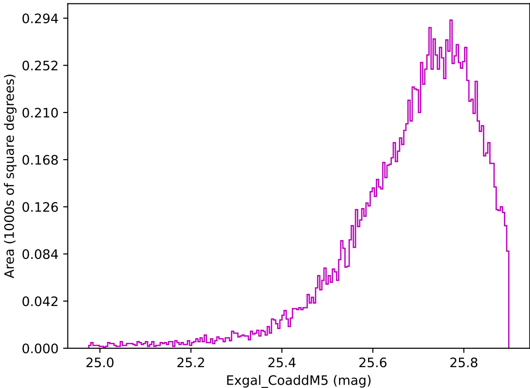
ddf_acor_sf15_lsf20_lsr20_v3.4_10yrs WFD z band: Exgal_CoaddM5
