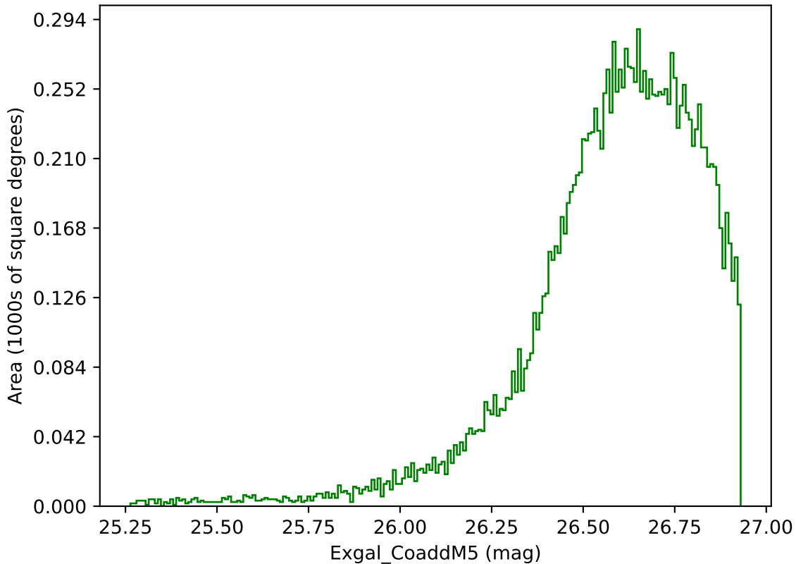
ddf_acor_sf15_lsf20_lsr20_v3.4_10yrs WFD g band: Exgal_CoaddM5
