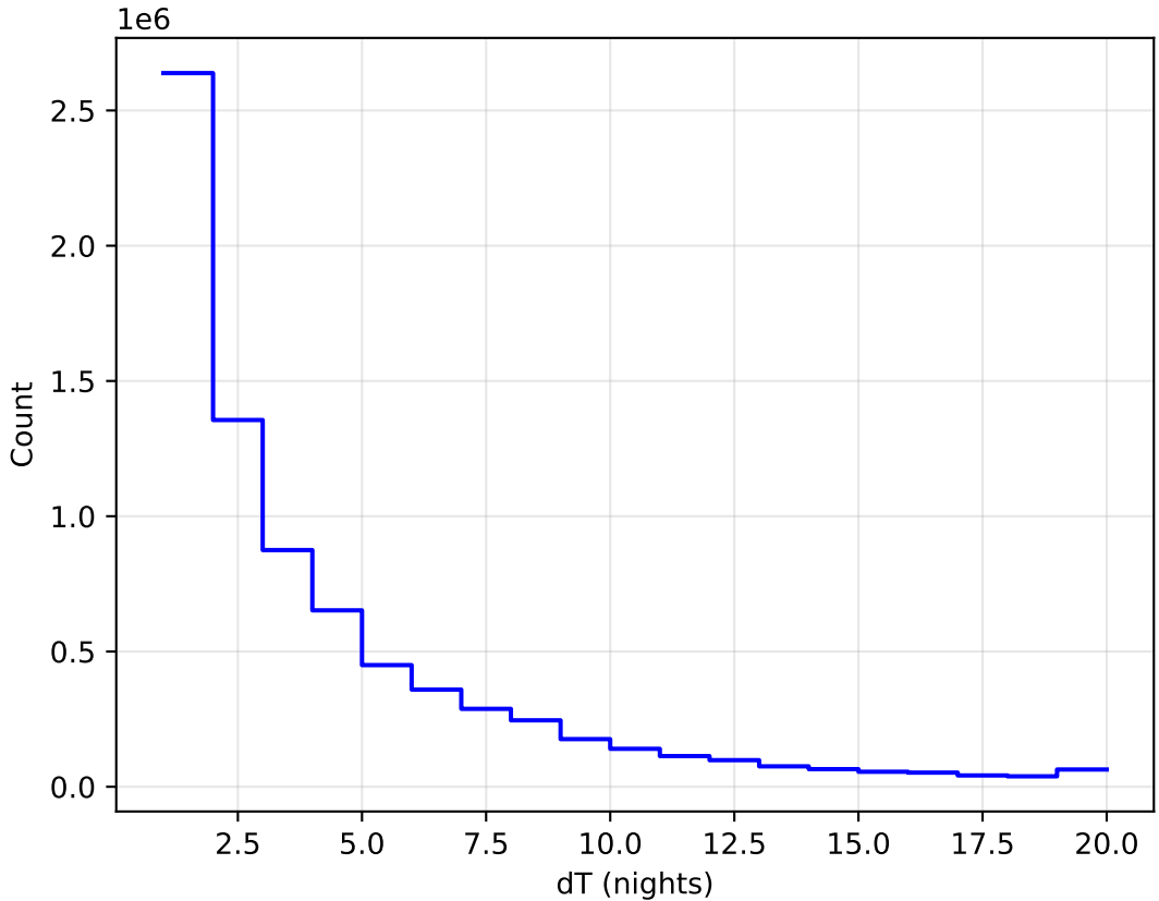
ddf_acor_sf15_lsf20_lsr20_v3.4_10yrs WFD all bands: DeltaNight Histogram
