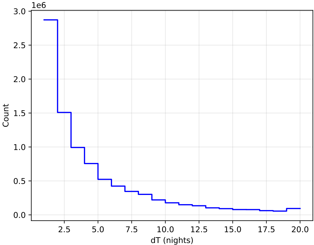
ddf_acor_sf15_lsf20_lsr20_v3.4_10yrs All sky all bands: DeltaNight Histogram
