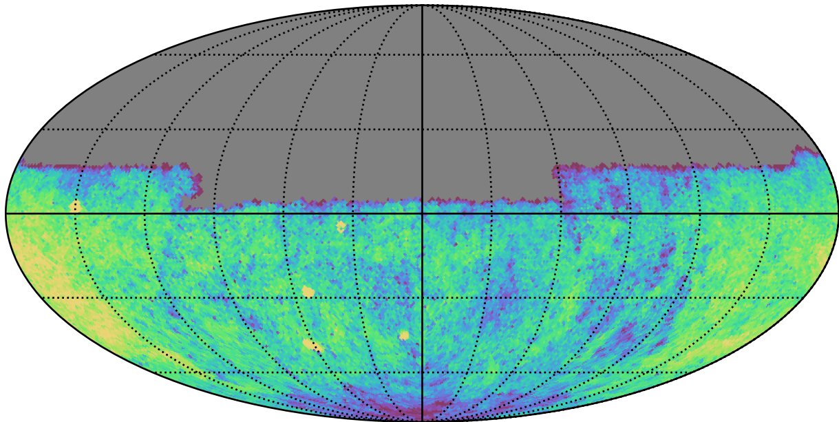
ddf_acor_sf15_lsf20_lsr20_v3.4_10yrs Yr 1 u band: CoaddM5
