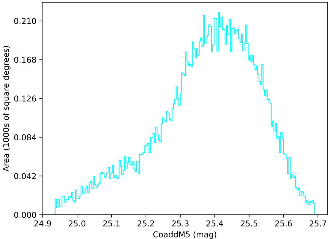
ddf_acor_sf15_lsf20_lsr20_v3.4_10yrs WFD u band: CoaddM5
