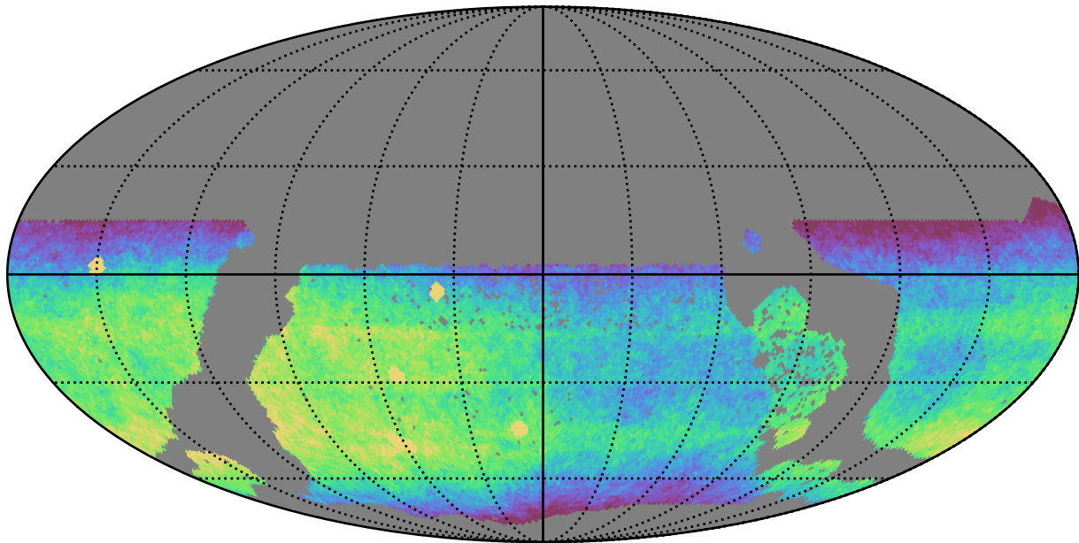
ddf_acor_sf15_lsf20_lsr20_v3.4_10yrs WFD r band: CoaddM5
