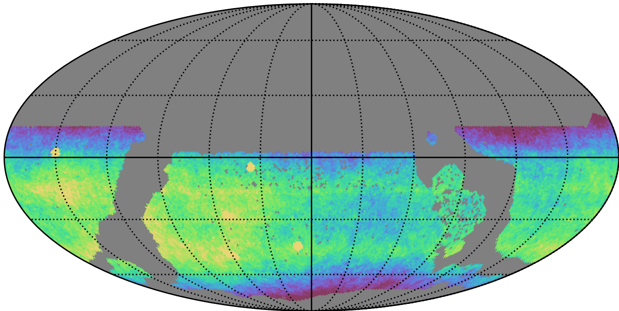
ddf_acor_sf15_lsf20_lsr20_v3.4_10yrs WFD i band: CoaddM5
