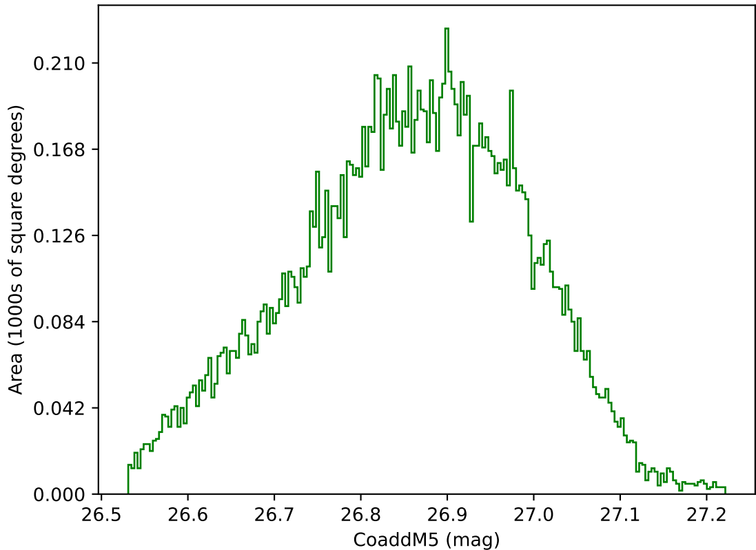
ddf_acor_sf15_lsf20_lsr20_v3.4_10yrs WFD g band: CoaddM5
