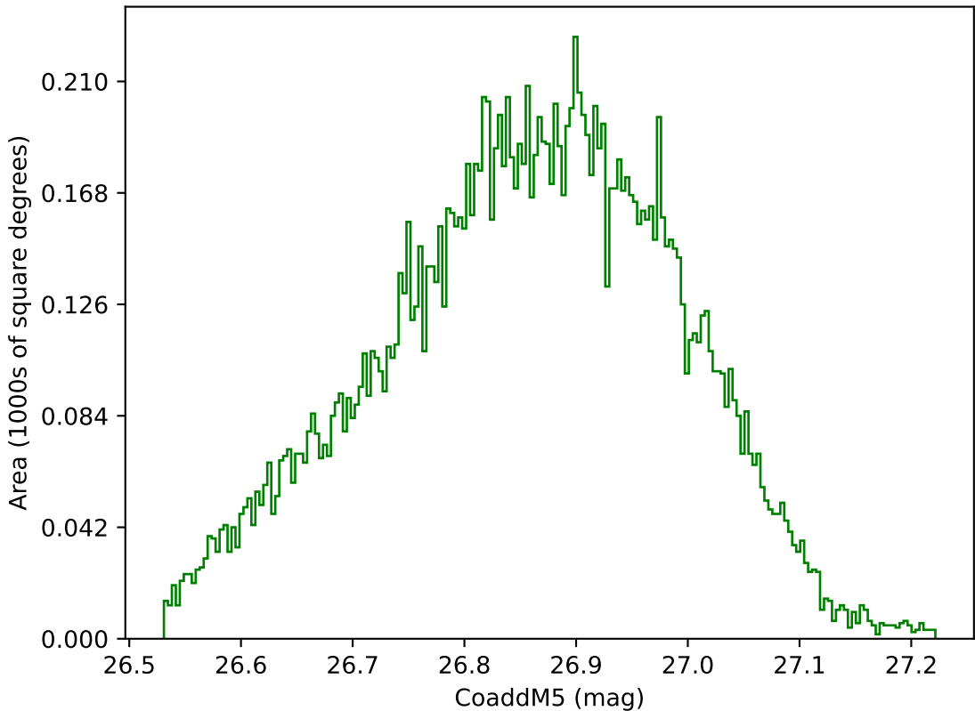
ddf_acor_sf15_lsf20_lsr20_v3.4_10yrs WFD g band: CoaddM5
