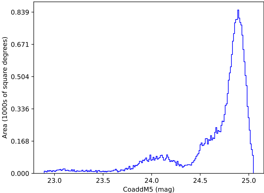
ddf_acor_sf15_lsf20_lsr20_v3.4_10yrs All sky y band: CoaddM5
