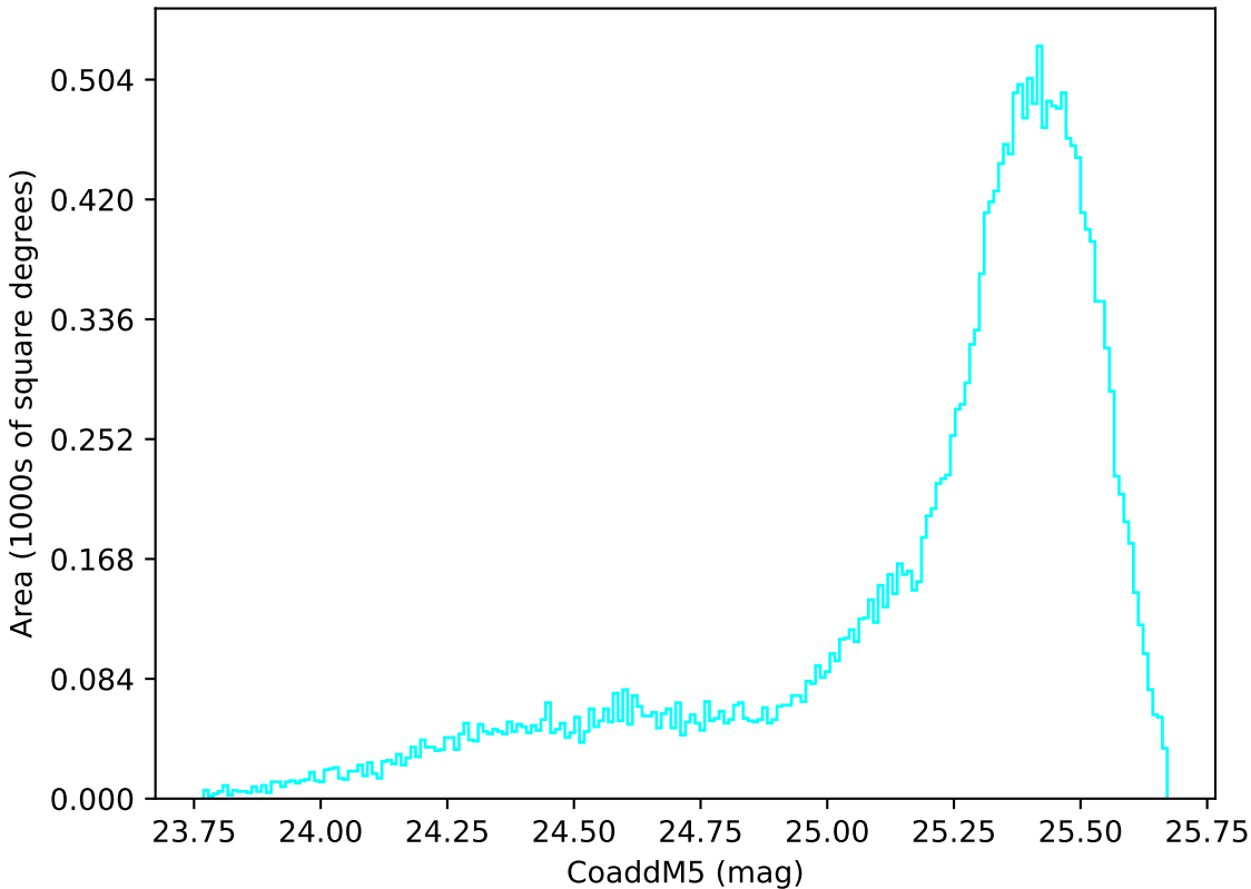
ddf_acor_sf15_lsf20_lsr20_v3.4_10yrs All sky u band: CoaddM5
