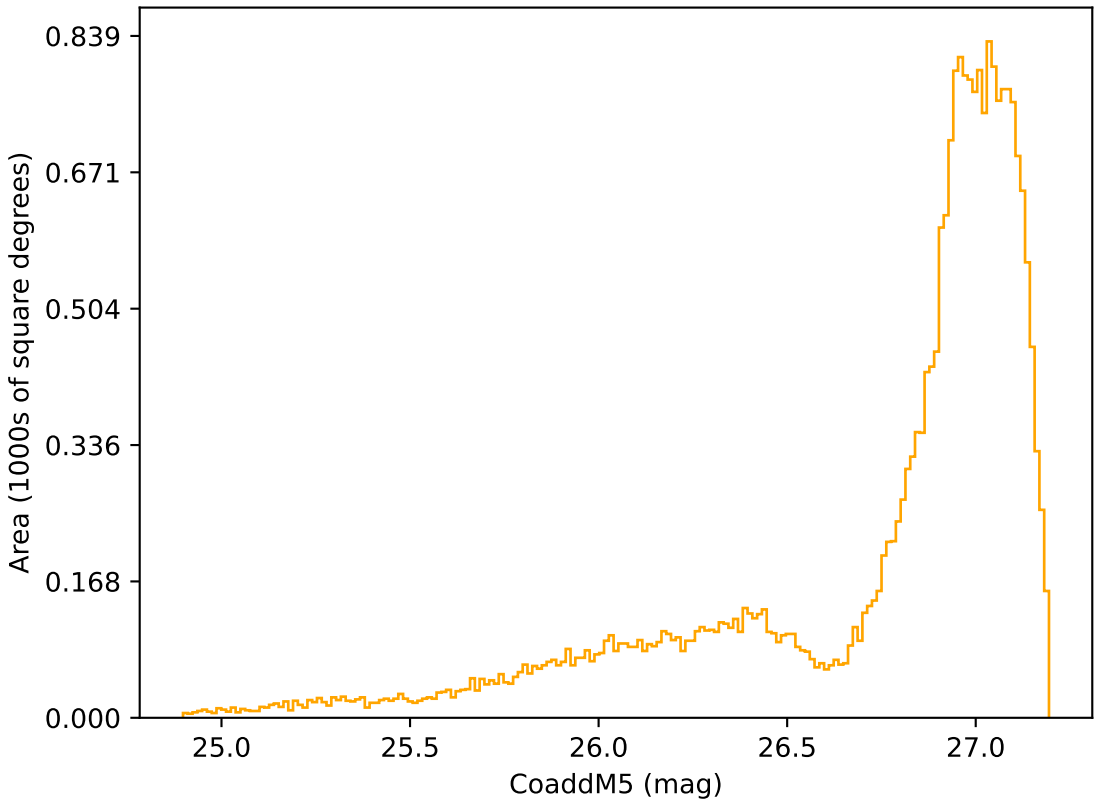
ddf_acor_sf15_lsf20_lsr20_v3.4_10yrs All sky r band: CoaddM5
