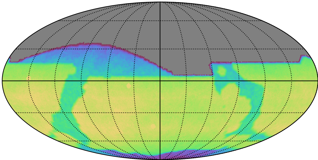
ddf_acor_sf15_lsf20_lsr20_v3.4_10yrs All sky i band: CoaddM5
