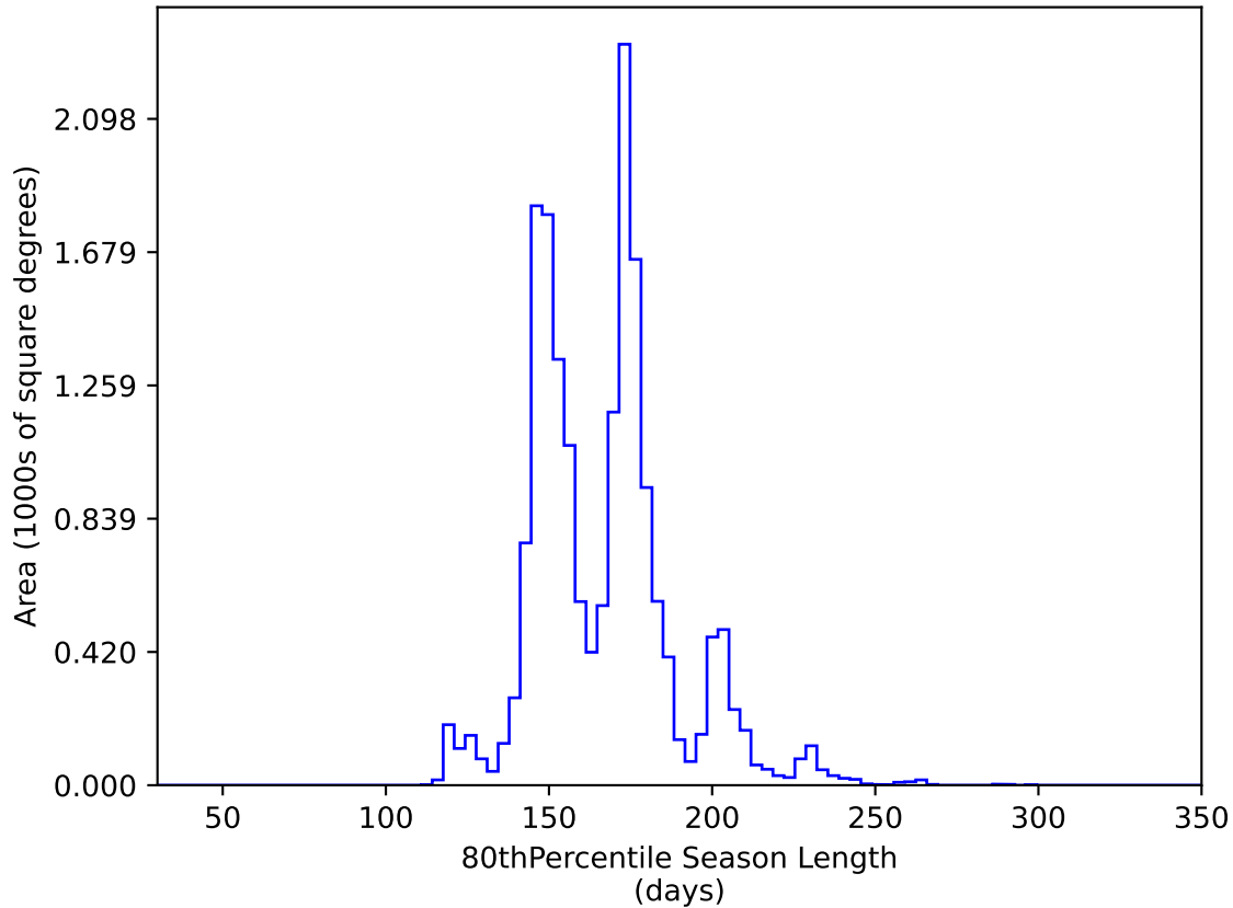
ddf_acor_sf15_lsf20_lsr20_v3.4_10yrs WFD y band: 80thPercentile Season Length
