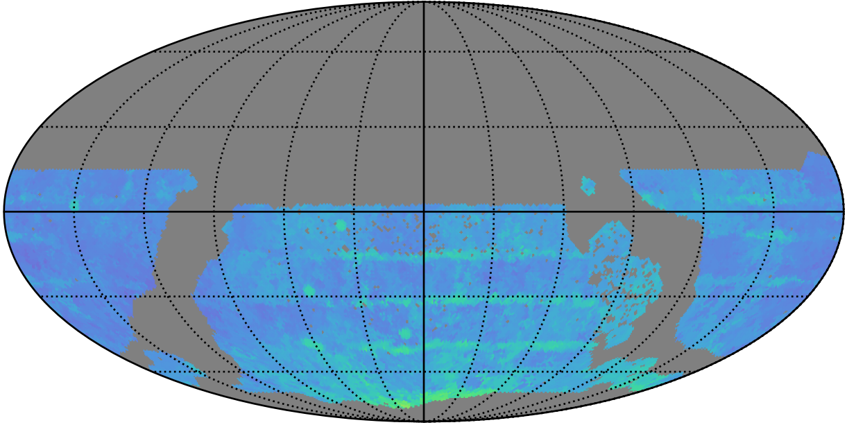
ddf_acor_sf15_lsf20_lsr20_v3.4_10yrs WFD r band: 80thPercentile Season Length
