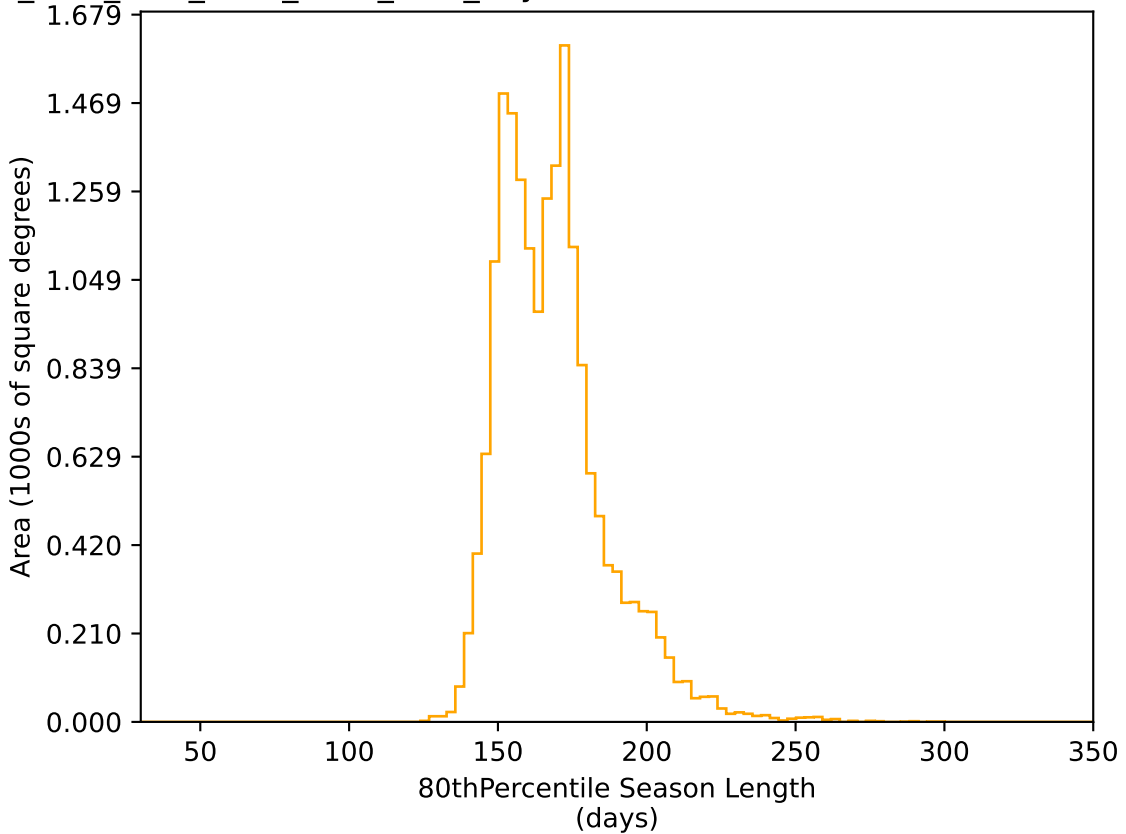
ddf_acor_sf15_lsf20_lsr20_v3.4_10yrs WFD r band: 80thPercentile Season Length
